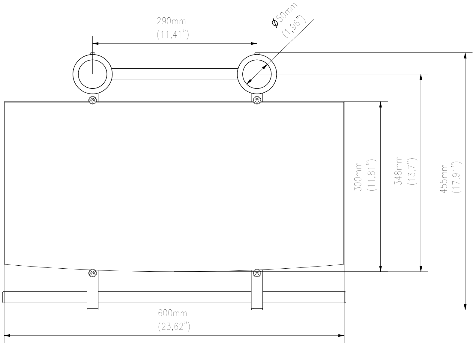
TOP VIEW
