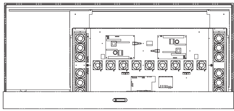
Main Shield - Open (H461SC)
