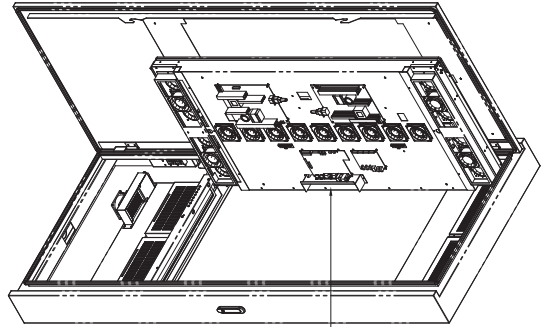
ISO VIEW (Main Shield - Open (H461SC))
