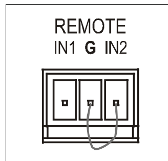
Figure 3: REMOTE Terminal Block Connector
