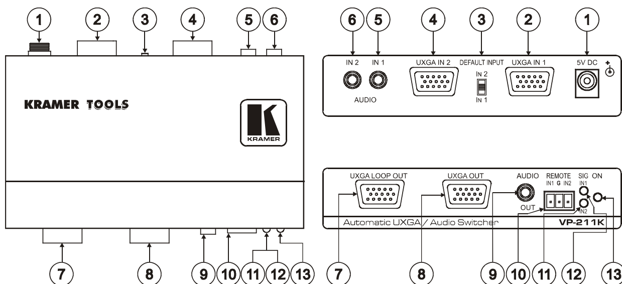
Figure 1: VP-211K Automatic UXGA / Audio Switcher
