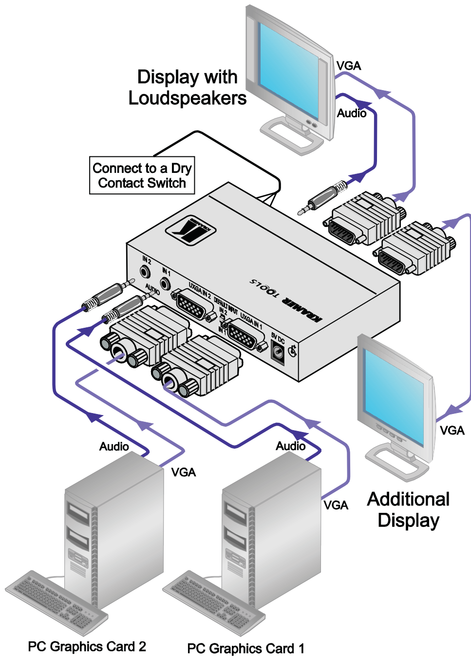
Figure 2: VP-211K Automatic UXGA / Audio Switcher Connections
