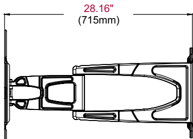
SIDE VIEW EXTENDED
