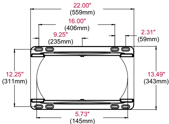
WALL PLATE
