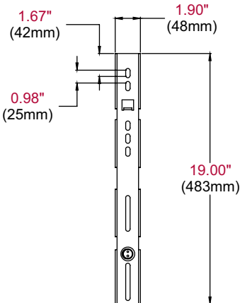
VERTICAL ADAPTER
