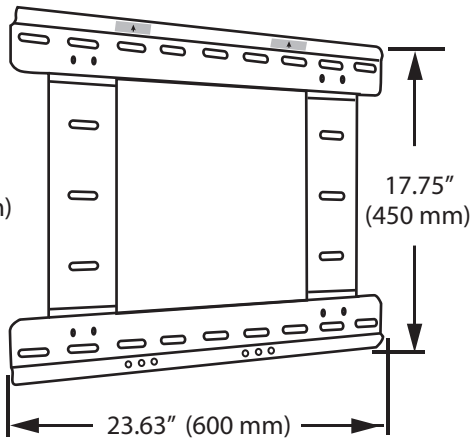
Wall Plate
