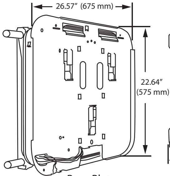
Base Plate
